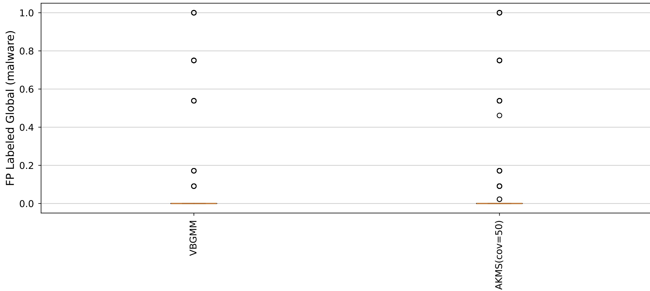
YARA Rules FP Labeled Global (malware) Distribution (Cluster5_Size23 dataset)
